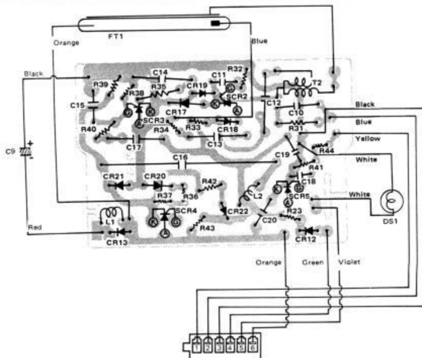
Figure 7. PC Board Foil Diagram
